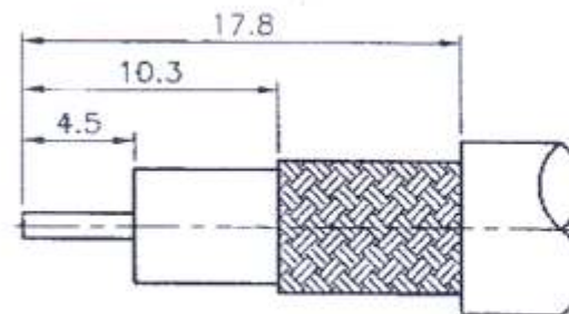
RECOMMENDED CABLE STRIPPING DIM'S (建議剝線尺寸)
